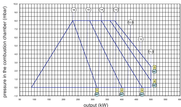
EXAMPLE OF PRE-CALIBRATION JOB 50/2
